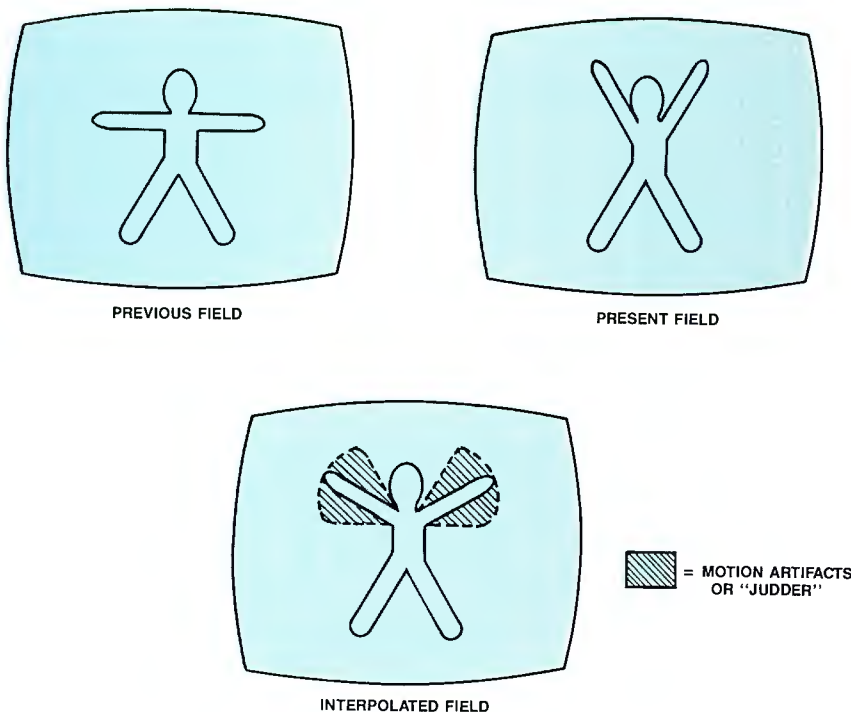
Figure 7. Motion artifacts, in some cases called "judder," occur when the exact position of an image between fields is ambiguous, hence unpredictable, due to video's low field-sampling rates.
