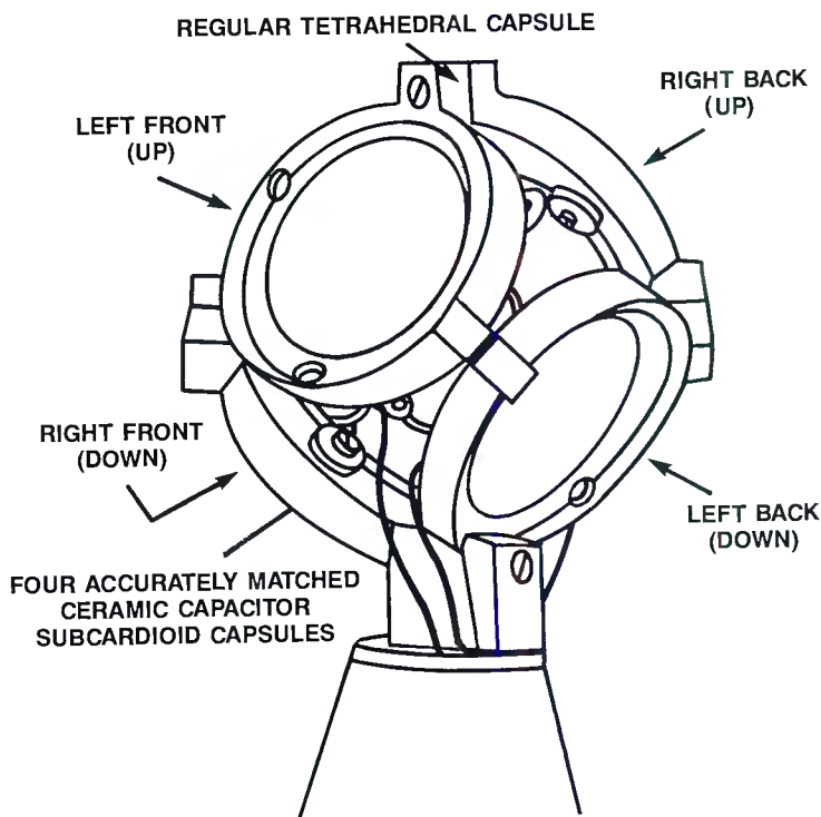
Figure 18. The Soundfield microphone uses four separate capsules to develop almost any type of polar pattern. If the four capsule outputs are recorded, the polar pattern can be varied in post-production work.
