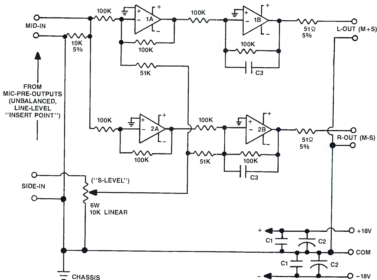
ACTIVE, LINE-LEVEL M-S MATRIX (UNBALANCED)
