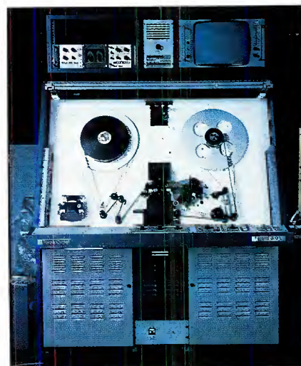
Rank Cintel's Ursa flying-spot scanner telecine uses advanced CRT design to provide special effects, zooms, pans and rotations. Effects are created by modifying the CRT beam's scanning patterns.
