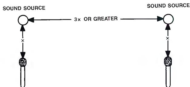
Figure 11. Observe the basic 3:1 rule when using more than one microphone. Remember that the rule applies for each microphone and sound source. Maintaining these distances can become a problem with more than a couple of microphones.
