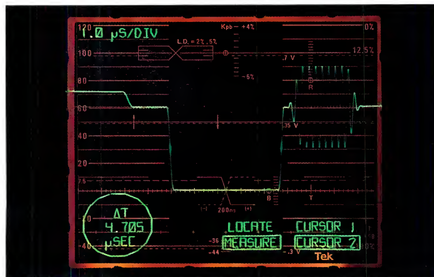
Figure 3. Time cursors, shown here as dots, allow timing intervals to be measured.
